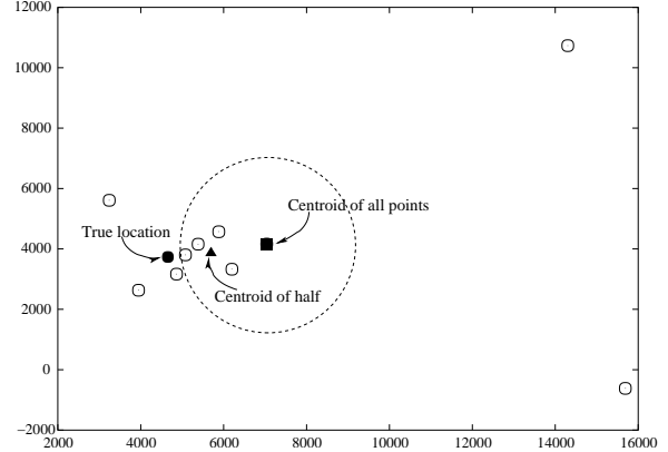
Fig. 9 REMOVING THE OUTLIERS FROM CENTROID COMPUTATION
