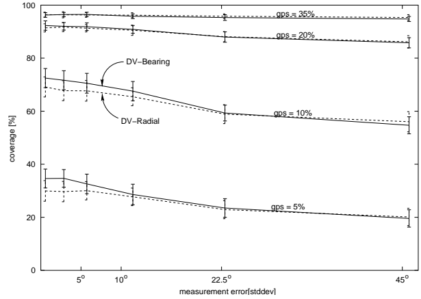
Fig. 14 COVERAGE
