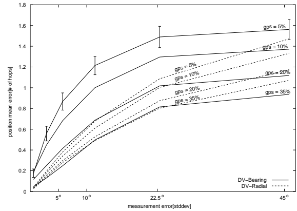
Fig. 11 POSITIONING ERROR
