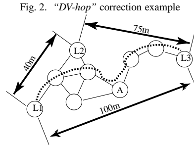
Fig. 2. “DV-hop” correction example
