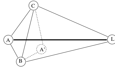
Fig. 2. “DV-hop” correction example
